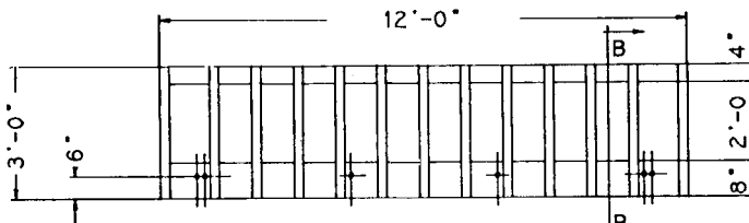
PC 32115 (3 X 12) Wt. = 335 Lbs.
