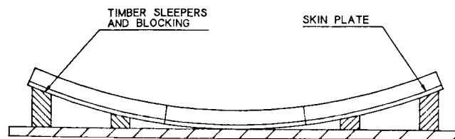
INSIDE GANG ASSEMBLY
