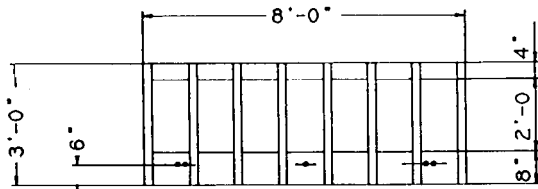
PC 32114 (3 X 8) Wt. = 214 Lbs.
