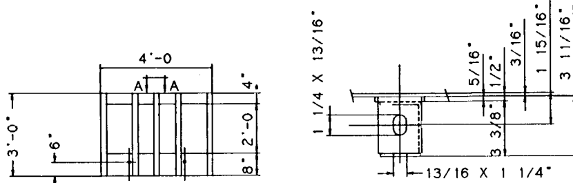
PC 32113 (3 X 4) Wt. = 129 Lbs. VIEW A-A
