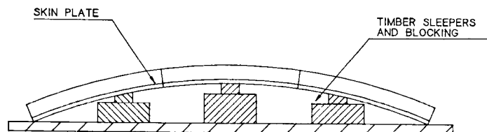
OUTSIDE GANG ASSEMBLY
