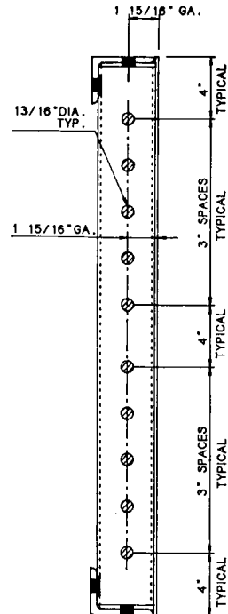
INTERIOR STIFFENER HOLE PATTERN
