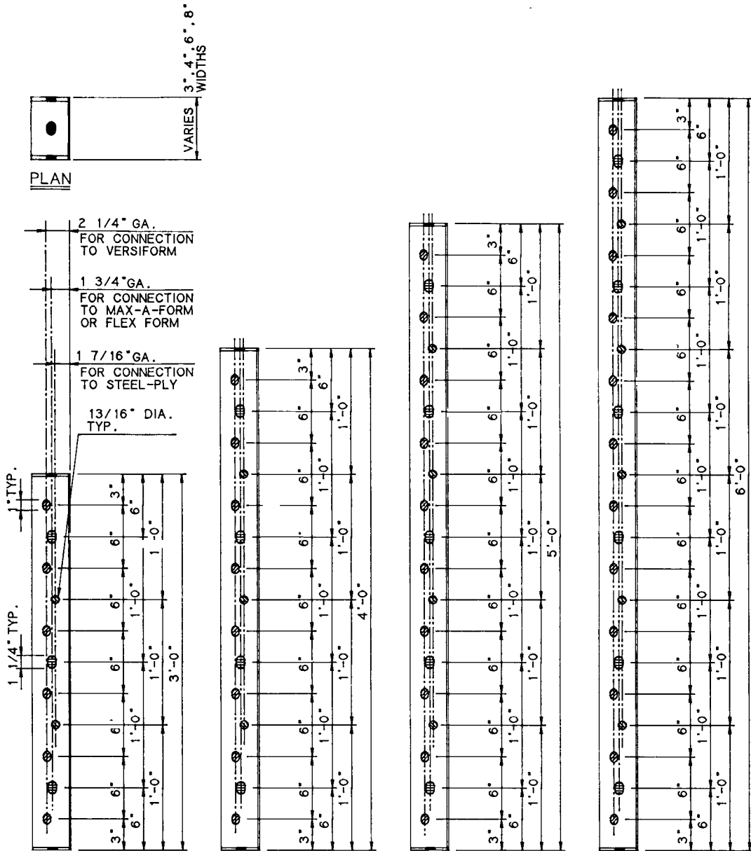
FILLER PANEL HOLE PATTERN
