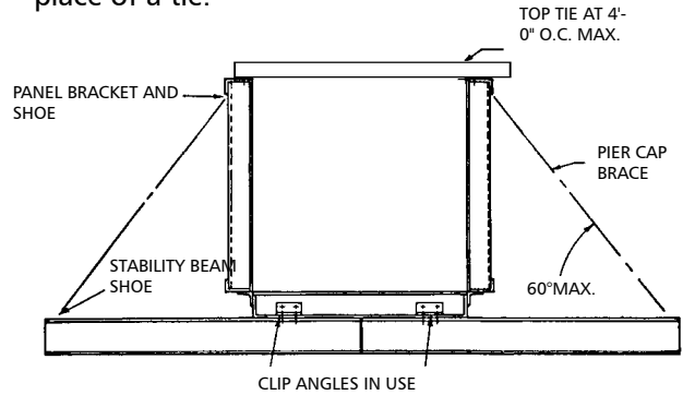
Stability Beam attached to Soffit
