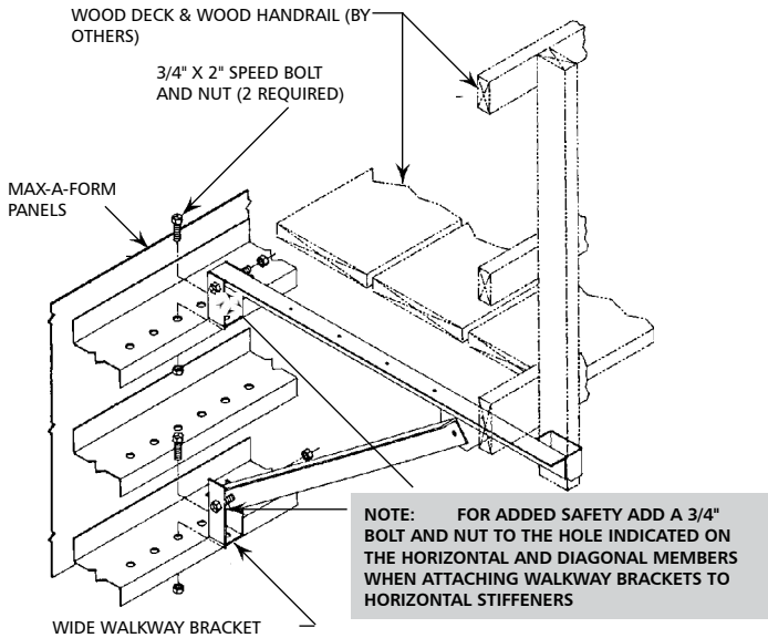
Wide Walkway Bracket Installation for Horizontal Stiffeners
