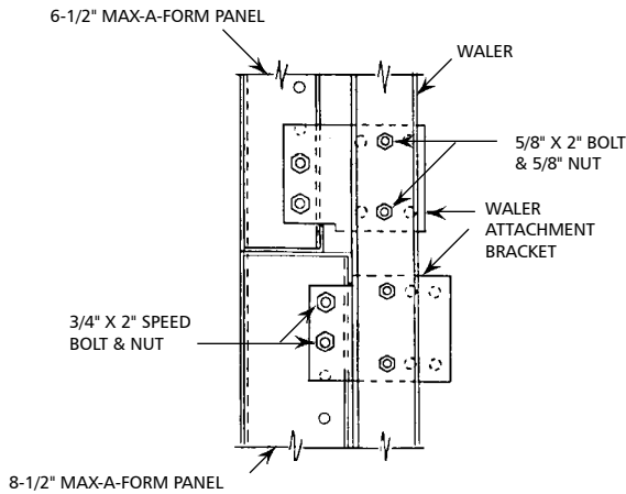
Stacking for Alignment Waler
