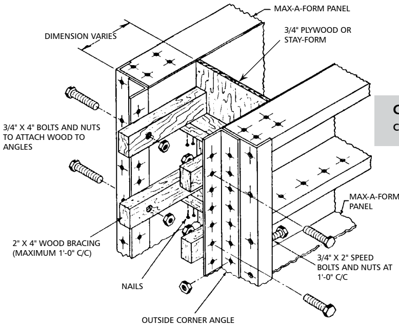
Outside Corner Angles used for End Bulkheads Maximum width 2'-0"
