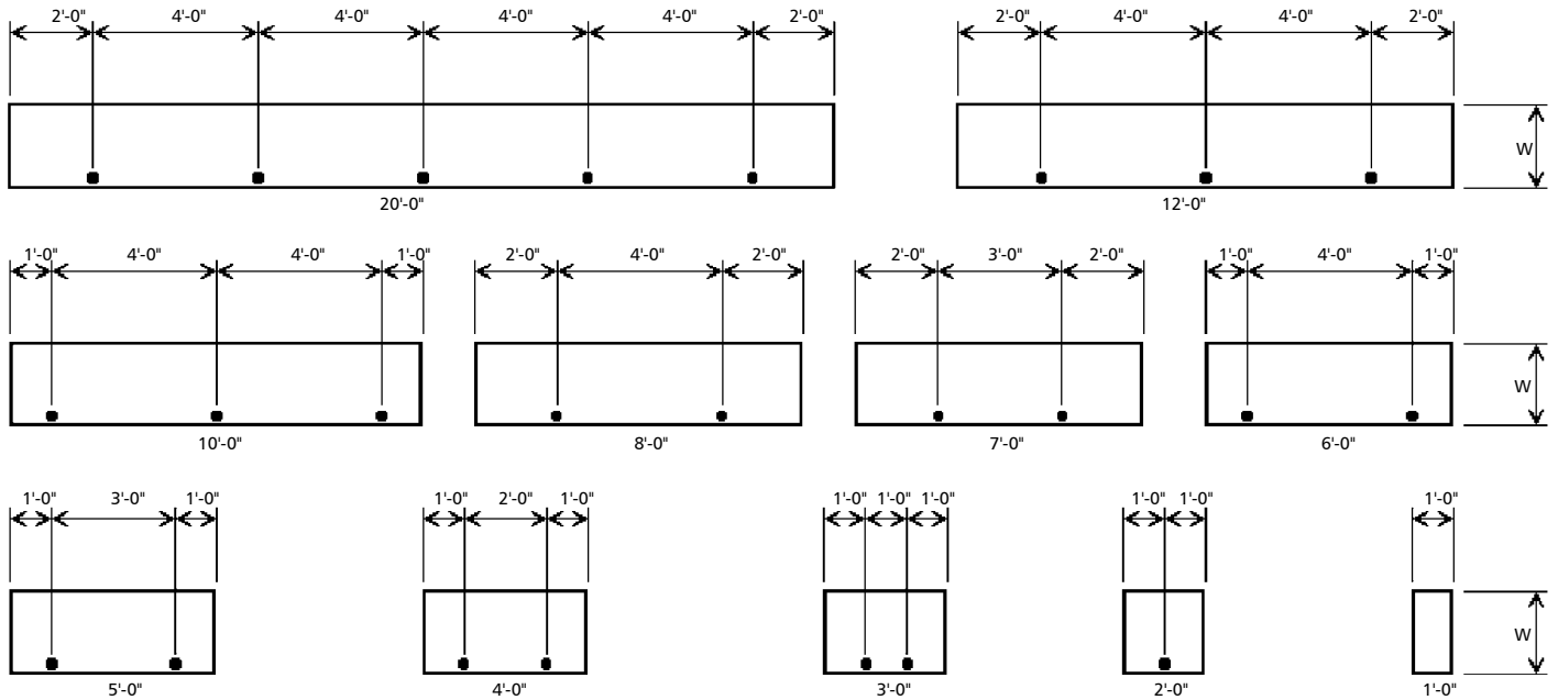
Tie Locations for Max-A-Form Panels
