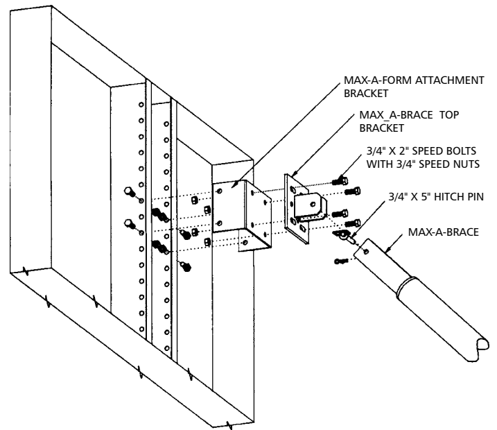
Max-A-Form Attachment Bracket and Max-A-Brace Top bracket connection to Max-A-Form panel with vertical stiffeners
