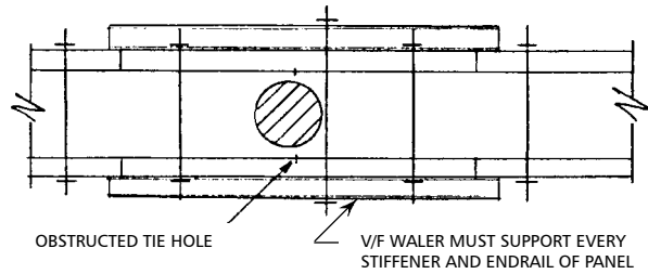
Using a Versiform Waler to Avoid Obstructions
