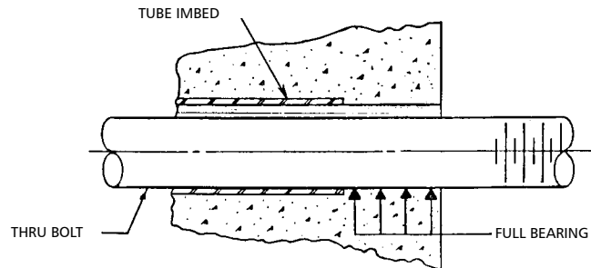
Section - Thru-Bolt Inserted
