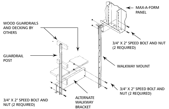
Max-A-Form Hanging Scaffold Erection (Vertical Stiffener Configuration)
