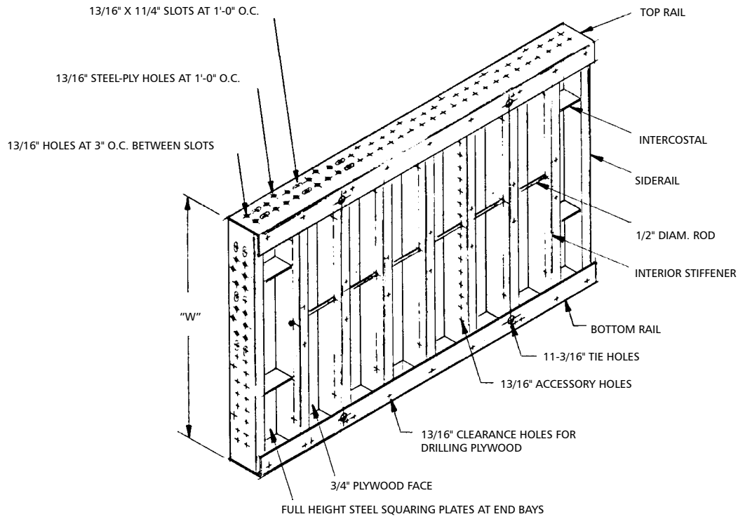
Max-A-Ply panel
