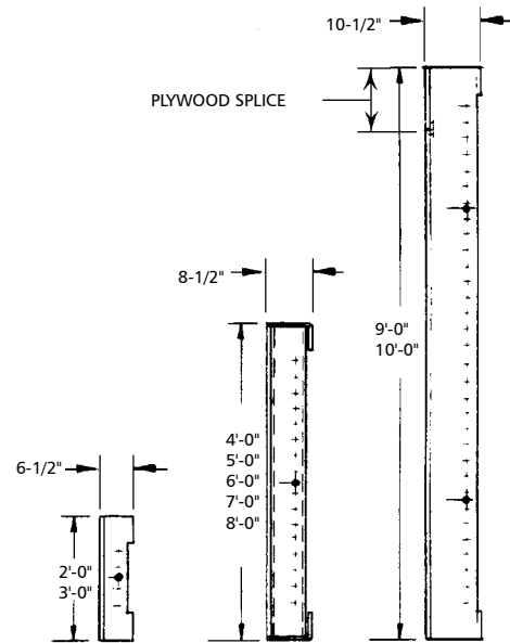
Panel Elevation A
