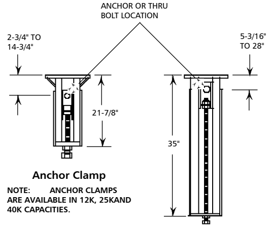
Adjustable Anchor Clamp
