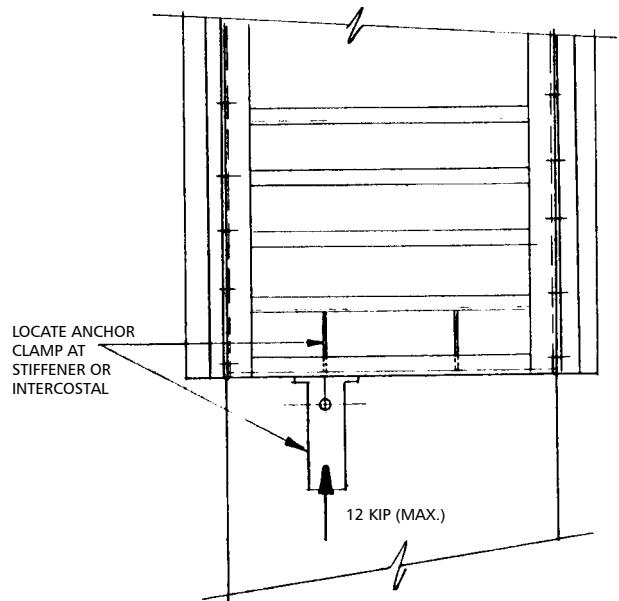
Elevation view (Support Limitations)
