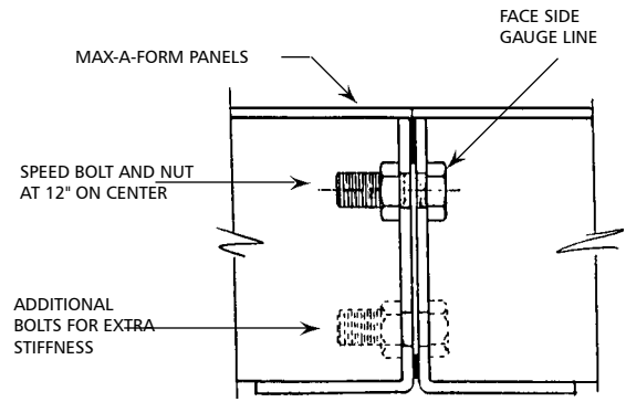
Max-A-Form Panel-To-Panel Bolt Connection
