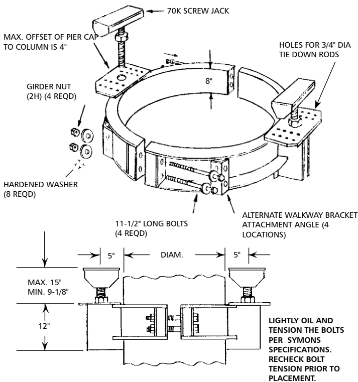
Circular Friction Collars
