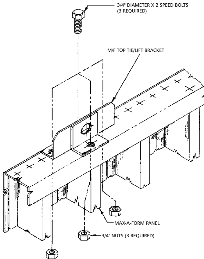
Max-A-Form Top Tie/Lift Bracket Installation
