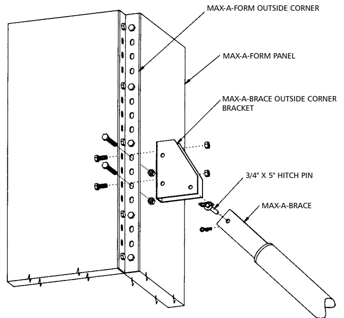
Max-A-Brace Outside Corner Bracket Connection to Max-A-Form Column Form
