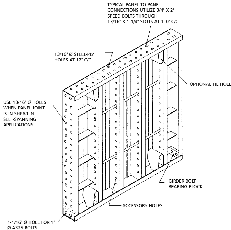
Typical Panel
