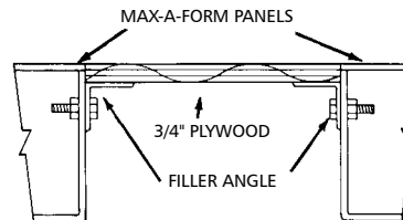
3/4" Plywood without 2" x 4" wood backing
