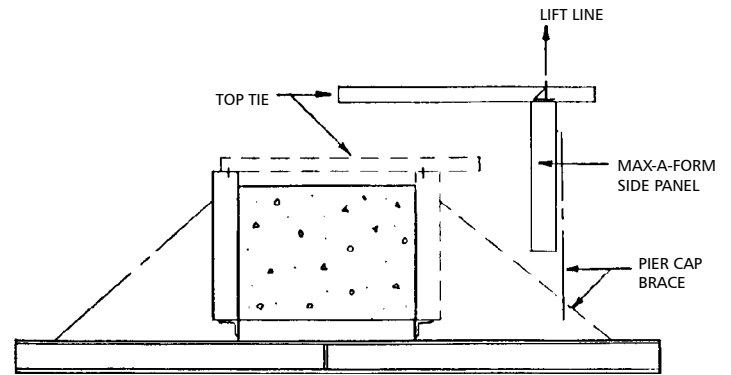
"I" Section Pick ("L" Section supported by Screw Jacks)
