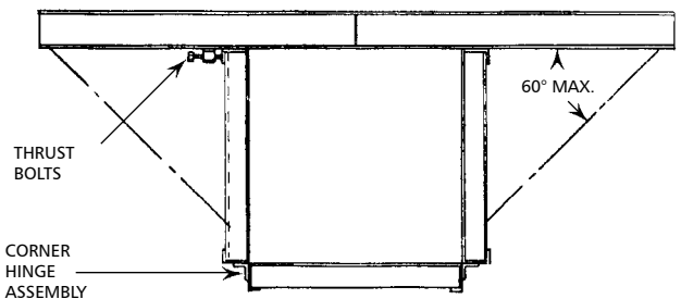
Stability Beam attached to Side Panels
