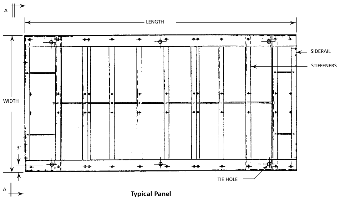
Typical Panel
