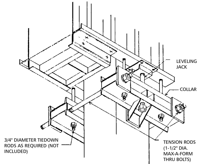
20 KIP Square Friction Collar
