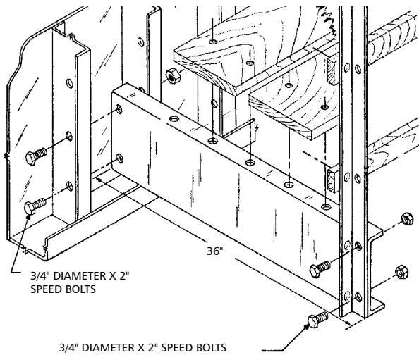
Alternate Walkway Bracket Installation
