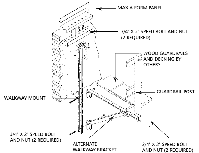
Max-A-Form Hanging Scaffold Erection (Horizontal Stiffener Configuration)
