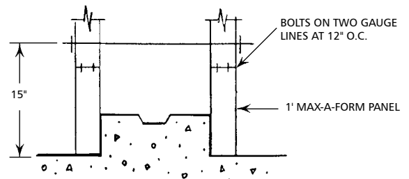
Raised Form
