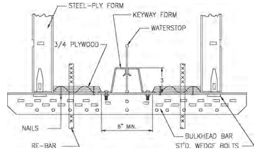
Keyway Bulkhead
