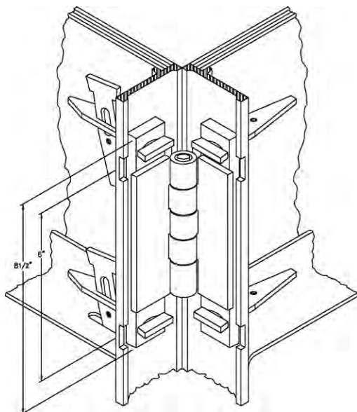
Column Hinge Installation
