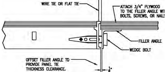
Typical Filler Angle Attachment
