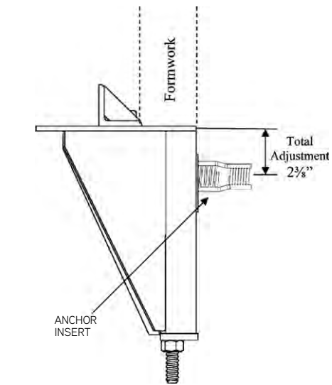
Typical Multi-Shear Wall Bracket Installation
