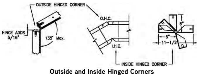
Outside and Inside Hinged Corners
