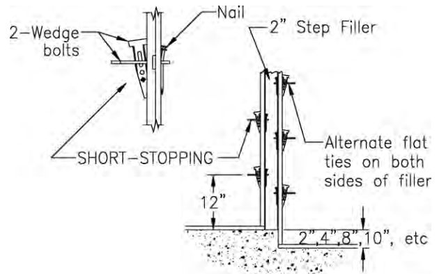
Flat Ties Only Typical Step Forming with Flat Ties
