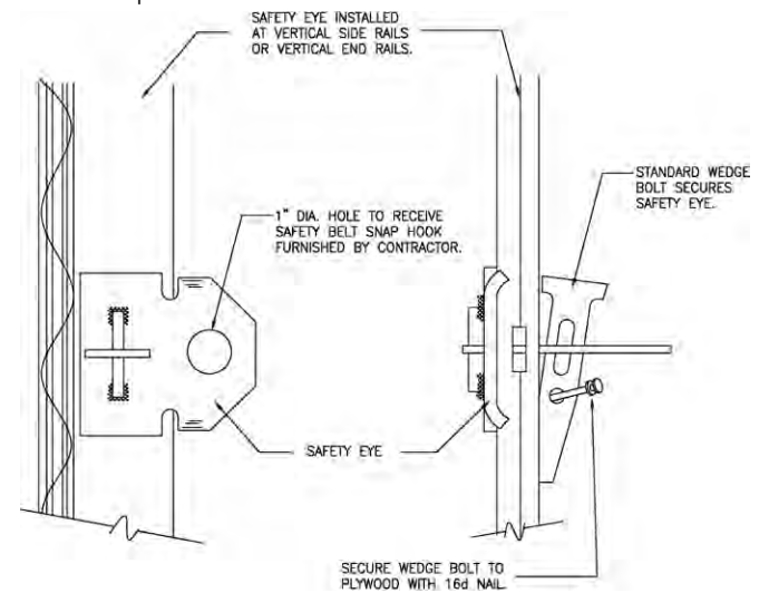
Safety Eye Installation
