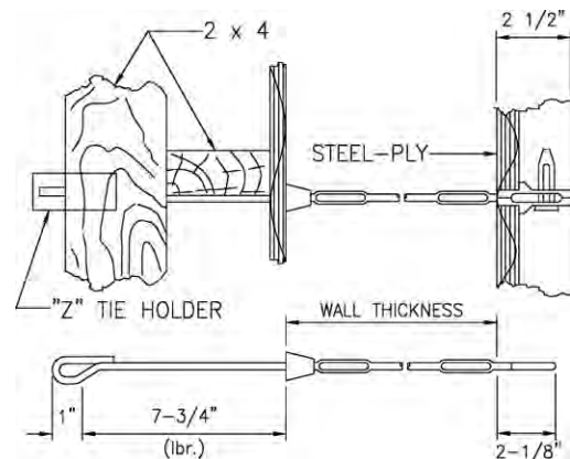
#2 Cone Tie
