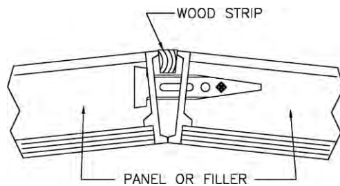
Installation of Wood Strips for Curves
